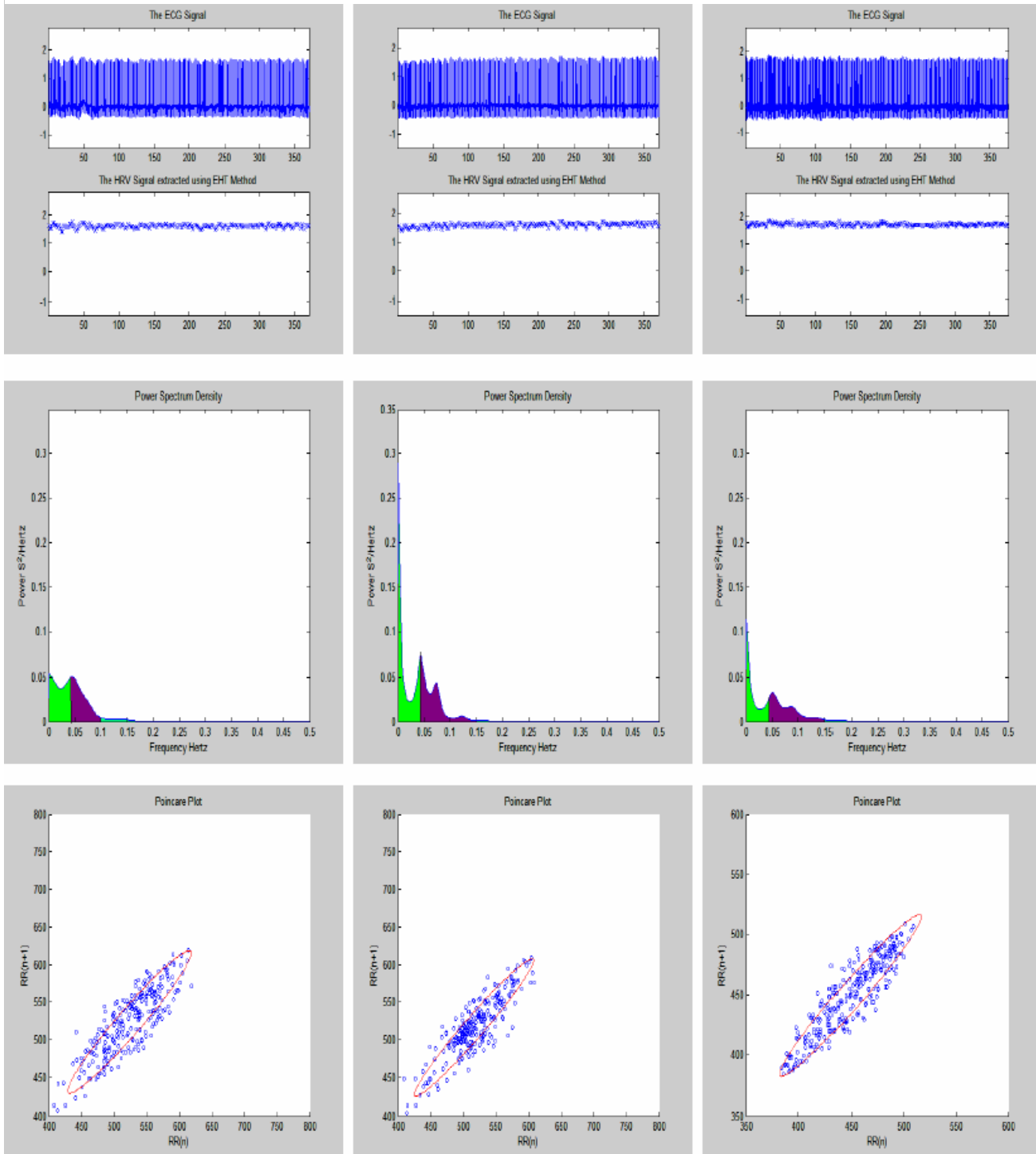
Figure 2. Exercise: Male Subject ECG & HRV signals (Upper traces) AR spectra of HRV (Middle traces) Poincare Plots (Lower traces) Spectral features and ApEn (Table)
